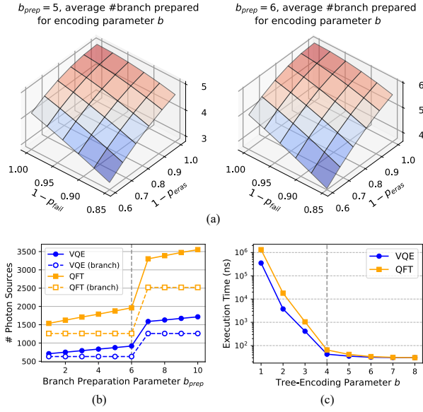
Fig. 5. (a) Average number of tree branches that successfully prepared for logical qubit encoding parameter b , when the preparation parameter b_{prep} = 5 and b_{prep} = 6 (by simulation). (b) Photon resource breakdown analysis for parameter b_{prep} , when given the maximum length of caterpillar is 30-qubit. Dashed lines represent the #photon sources used for branch preparation. (c) Execution time analysis for the tree-encoding parameter b , under a noise model that p_{fail} = 2\% and p_{eras} = 25\% .
