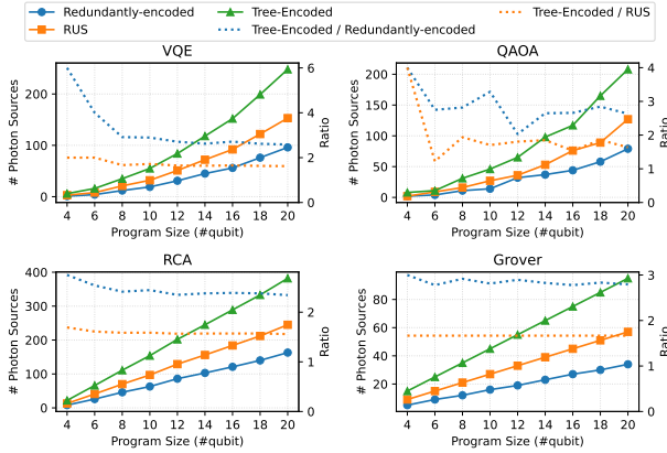
Fig. 9. Number of required photon sources comparison between tree-encoded scheme and baselines.
