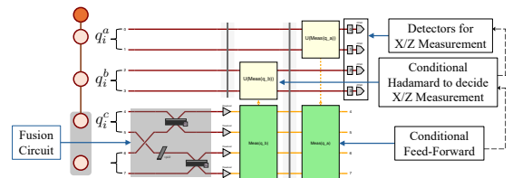
Fig. 13. The optical hardware circuit for tree-encoded fusion.
