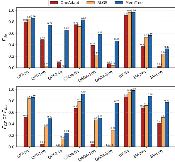
Fig. 11. Comparison on decoherence errors and CZ errors between OneAdapt [74], RLGS [38] and MemTree.
