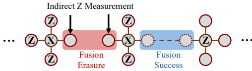
Fig. 7. Addressing erasure error in OneAdapt-ET.
